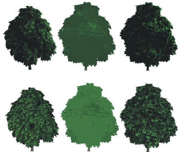
Figure 13 : Left column shows original geometry, middle column flat shaded Billboard Clouds, right column dynamically per-pixel lighted Billboard Clouds. Top and bottom row show different light directions.
