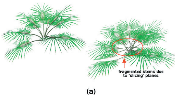
Figure 4: Billboard Cloud artifacts: (a) loss of continuity. (b) The front faces should ideally be simplified to one vertical plane. However, the dominant top and bottom planes preemptively simplify the front faces and leave a large hole in the front.
