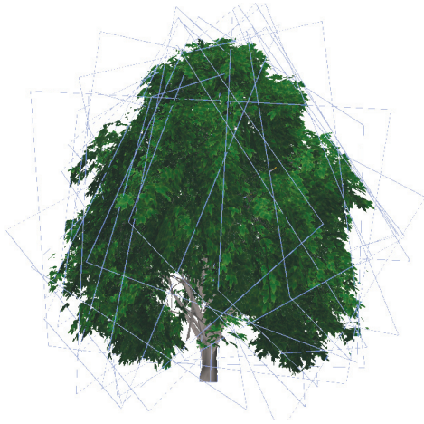
Figure 2: Billboard Cloud tree composed of 25 billboards (50 triangles). Original model consists of 159.853 triangles.
