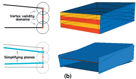
Figure 4: Billboard Cloud artifacts: (a) loss of continuity. (b) The front faces should ideally be simplified to one vertical plane. However, the dominant top and bottom planes preemptively simplify the front faces and leave a large hole in the front.
