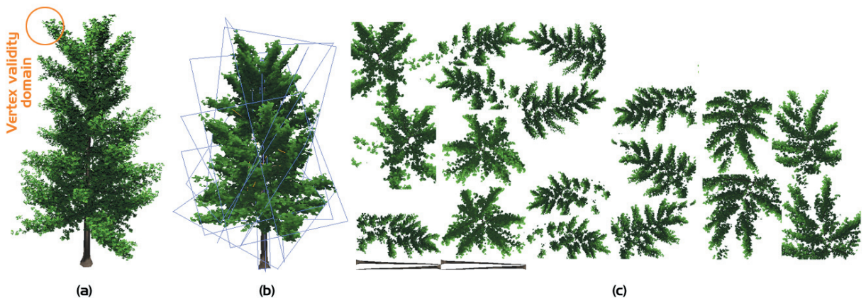
Figure 3: A 110,000 polygons tree model (a) simplified to 11 billboards (b). The error threshold is shown by the vertex validity domain. Billboard textures are depicted in (c).
