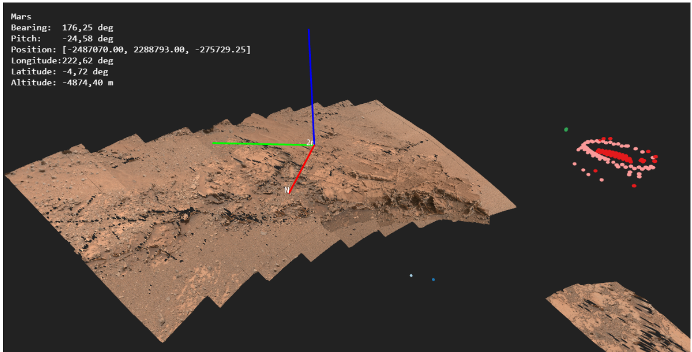
Figure 4: MSL product locations as dots of Mastcams (red), Navcams (blue), and ChemCam (green) in spatial context with the Garden City outcrop reconstruction. 3D data was derived from Mastcam images of the Sols 925, 926, and 929. Data Credits: NASA/CalTech/MSSS/ASU
