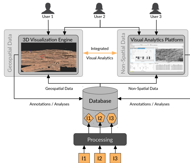
Figure 1: MINERVA architecture, the instrument teams use the generic importer tools (or in the case of vision the existing vision processing) to ingest mission data into the database (I1,I2,I3). From there it is available to the 3D Visualization Engine with integrated GIS functionality and the Visual Analytics Platform. Different users can share the same locations, observations, and launch visual analysis of different instruments at a time. A communication protocol allows the usage of visual analysis methods on spatial and non-spatial representations across applications.
